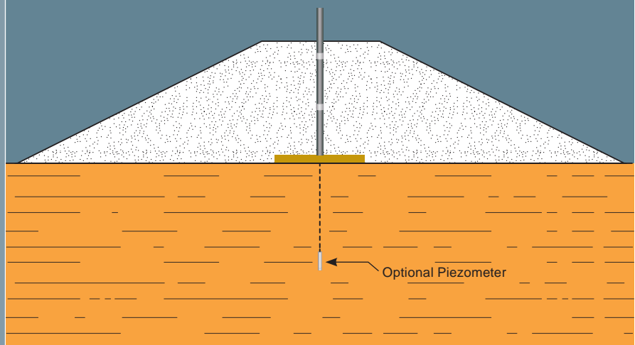
Typical installation
